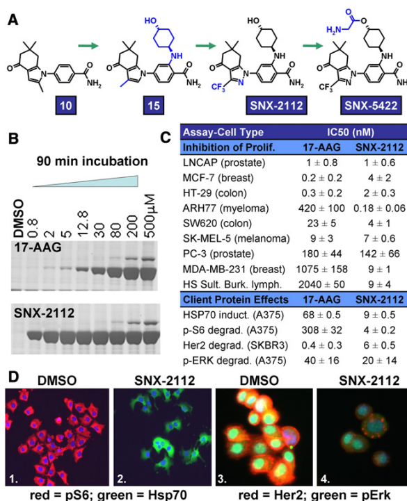
Figure 4. Identification and In Vitro Pharmacology of SNX-2112
