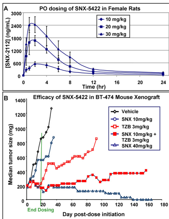
Figure 5. In Vivo Pharmacology of SNX-5422
