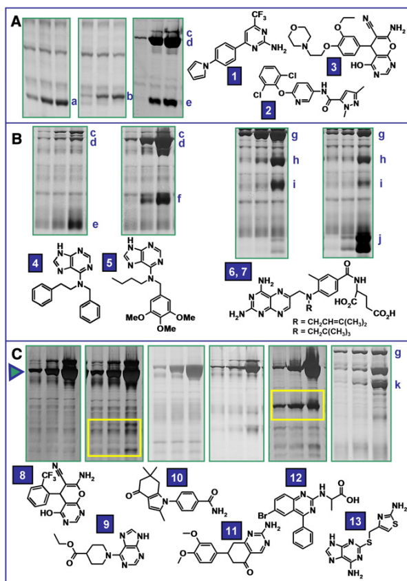
Figure 2. Screening a Targeted Library
