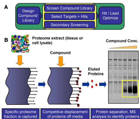
Figure 1. Overview of Chemoproteomics-Based Discovery Process
